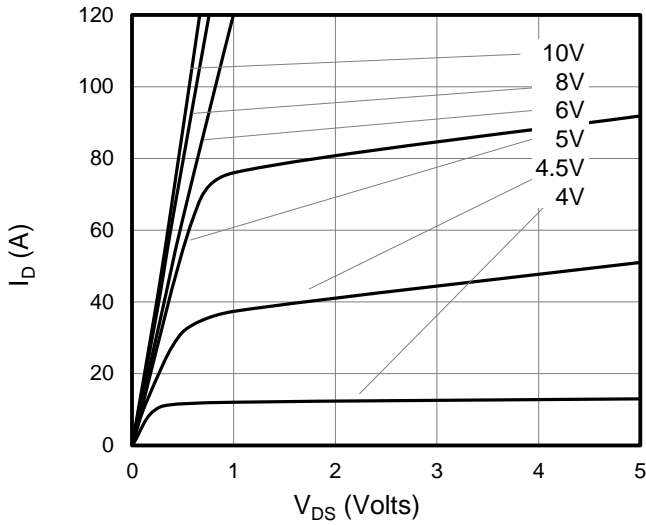
Figure 1: On-Region Characteristics
