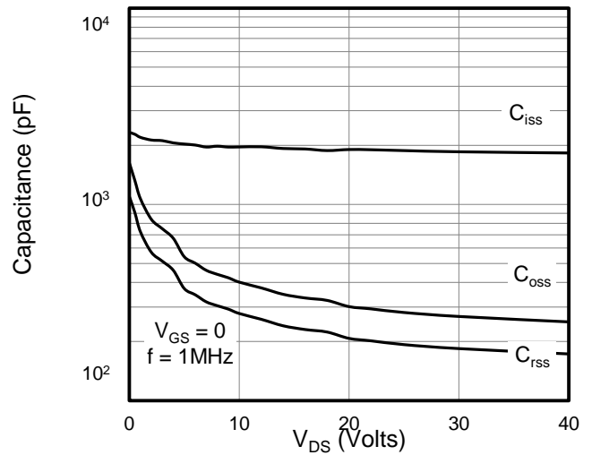
Figure 4: Capacitance Characteristics
