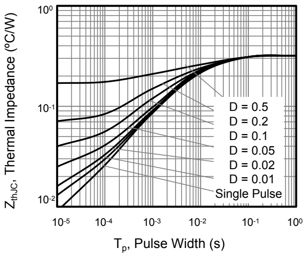
Figure 9. Transient Thermal Impedance For TO-263/TO-247
