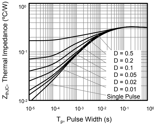
Figure 9. Transient Thermal Impedance For TO-247/TO-3PN
