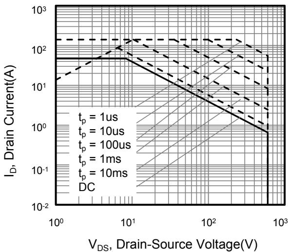
Figure 11. Safe Operation Area For TO-247/TO-3PN
