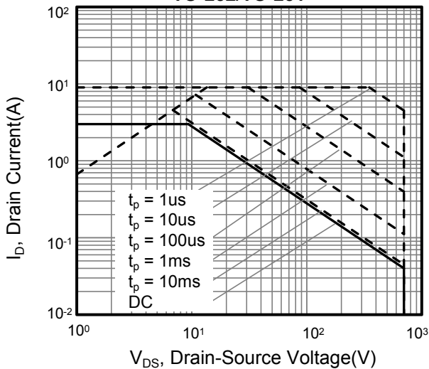
Figure 11. Safe Operation Area For TO-252/TO-251
