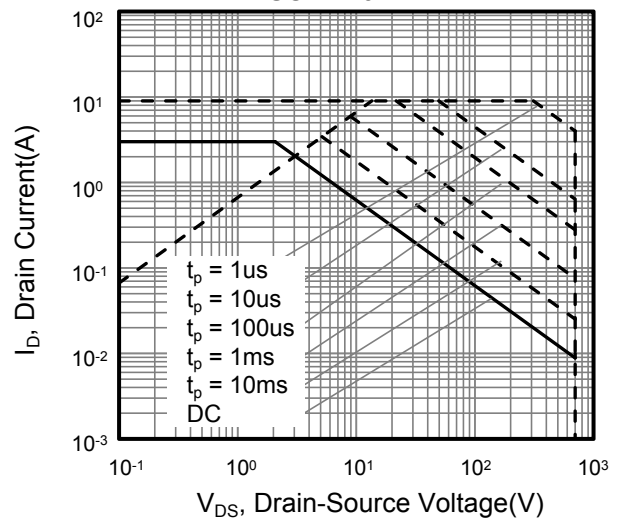
Figure 12. Safe Operation Area For SOT-223-2L
