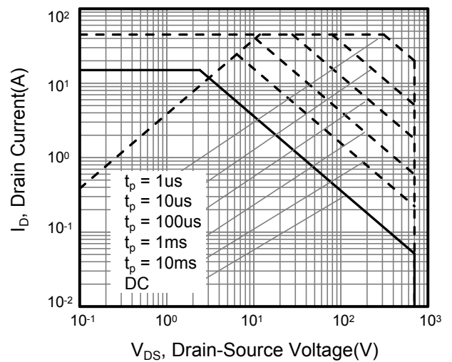
Figure 10. Safe Operation Area For TO-220F/TO-220FP-NL
