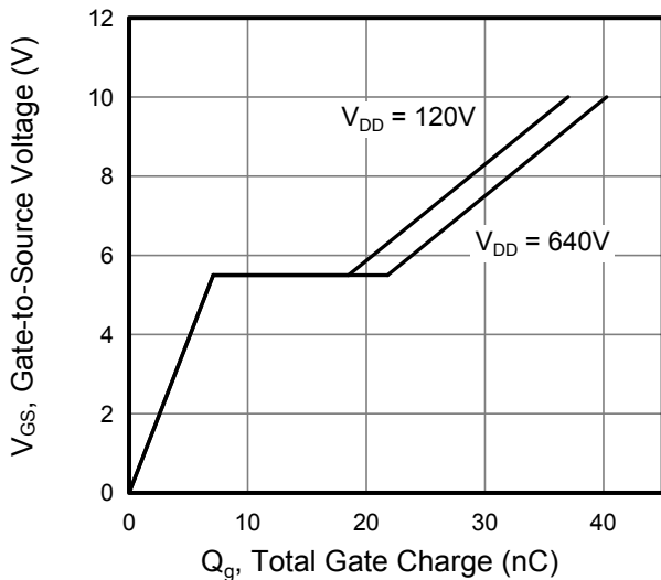
Figure 5. Gate Charge
