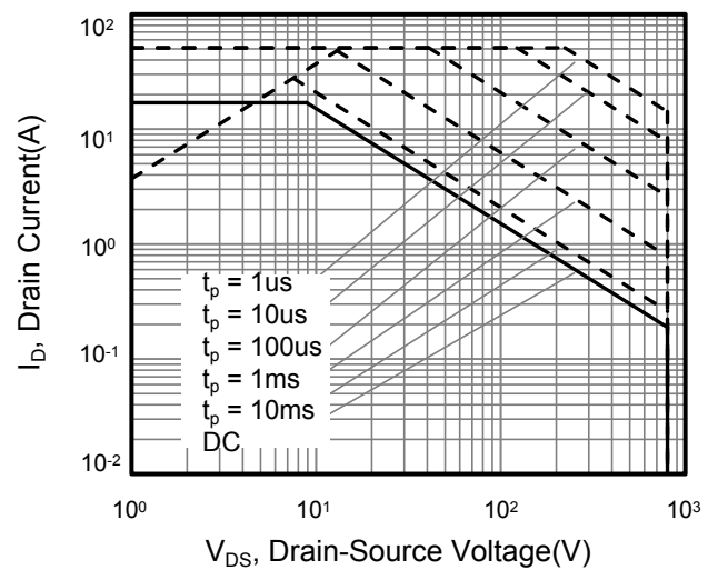
Figure 10. Safe Operation Area For TO-220/TO-247
