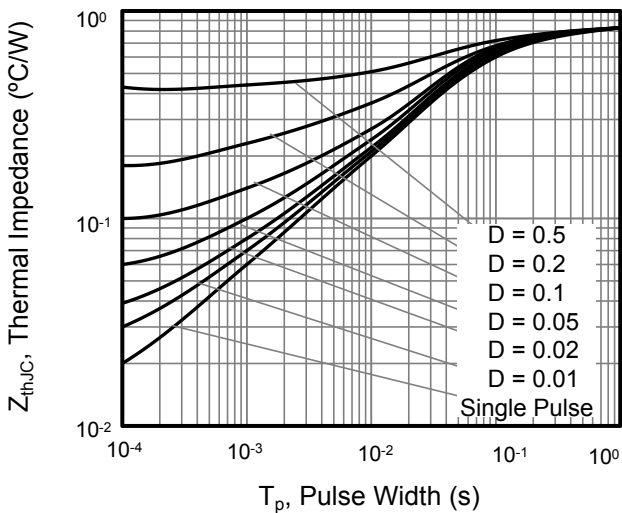
Figure 9. Transient Thermal Impedance For TO-220/TO-247
