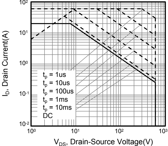
Figure 11. Safe Operation Area For TO-220/TO-3PN/TO-247
