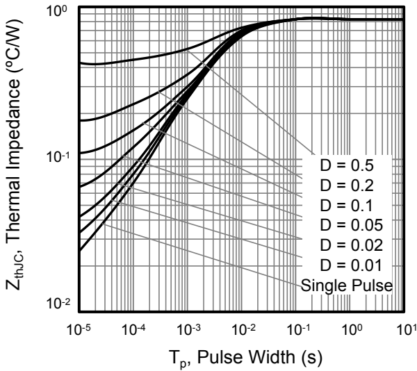
Figure 9. Transient Thermal Impedance For TO-220/TO-3PN/TO-247
