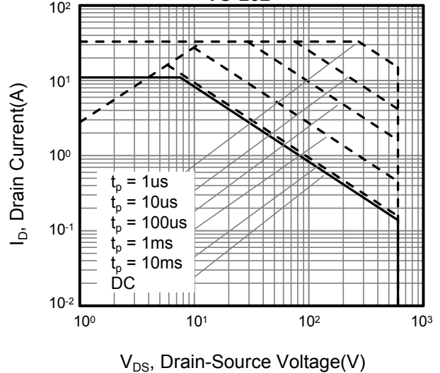
Figure 12. Safe Operation Area For TO-252
