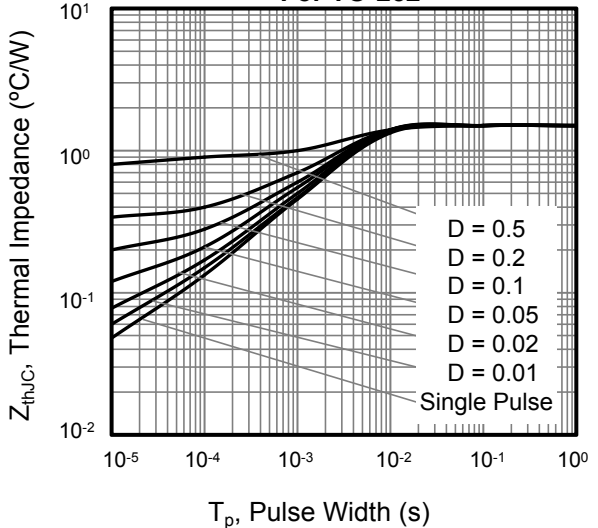
Figure 11. Transient Thermal Impedance For TO-252
