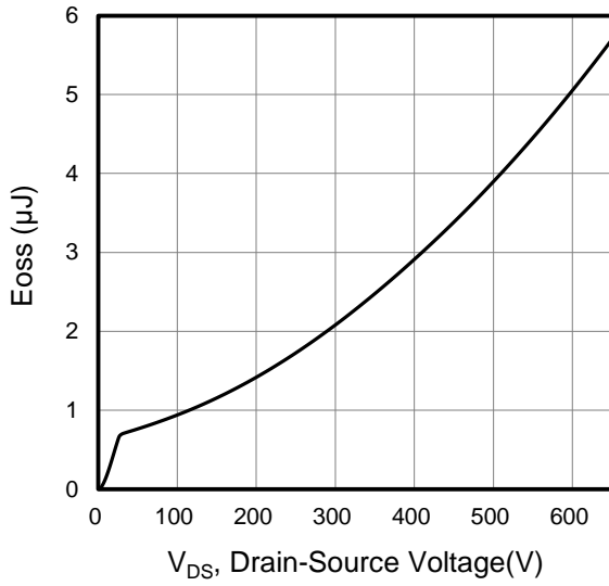
Figure 13. Typ. Coss Stored Energy
