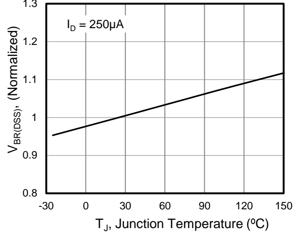
Figure 8. T Breakdown voltage vs. Junction Temperature
