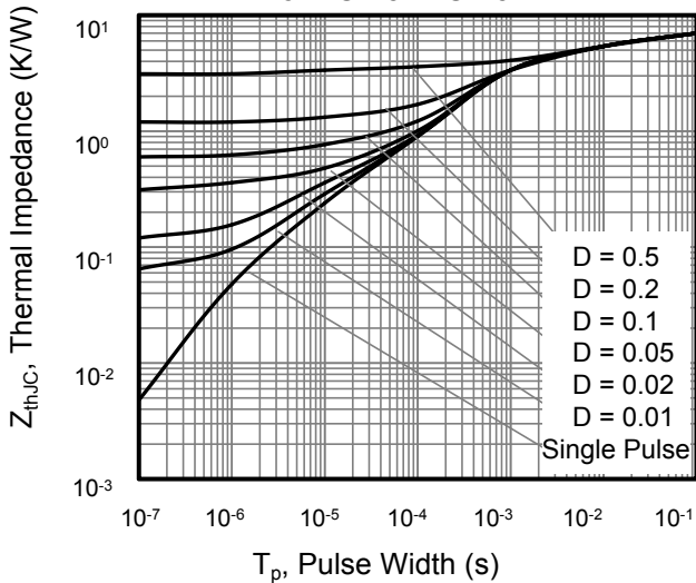
Figure 9. Transient Thermal Impedance For TO-251/TO-252
