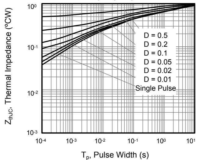
Figure 10. Transient Thermal Impedance For TO-220F
