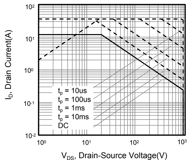
Figure 12. Safe Operation Area For TO-247
