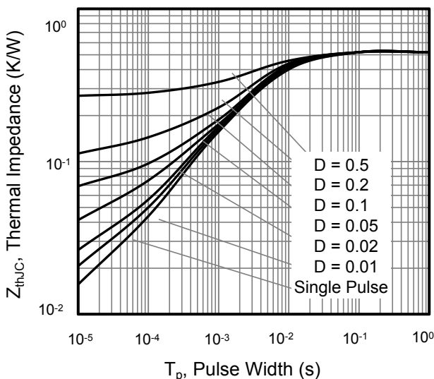
Figure 11. Transient Thermal Impedance For TO-247
