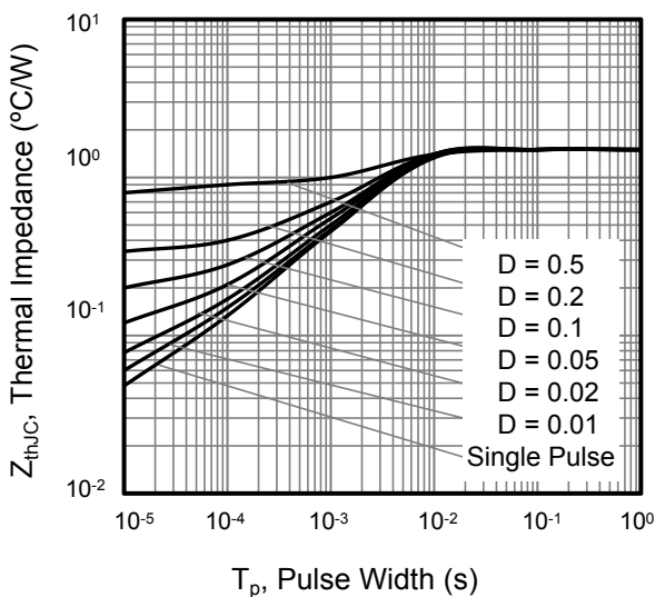
Figure 11. Transient Thermal Impedance TO-252
