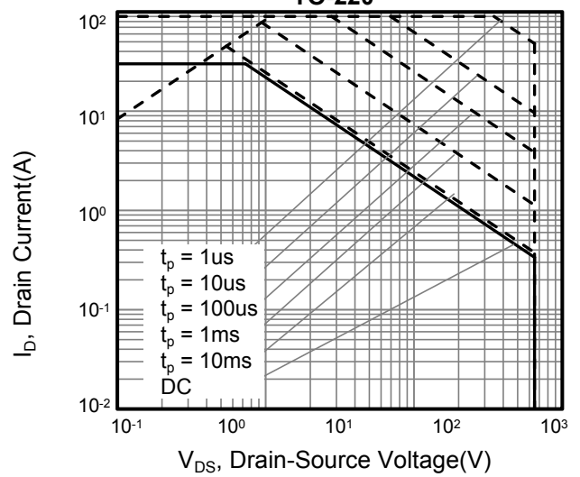
Figure 10. Safe operation area for TO-220
