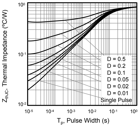
Figure 9. Transient Thermal Impedance DFN 8*8
