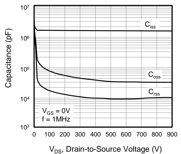
Figure 4. Capacitance
