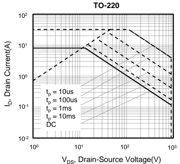
Figure 12. Safe operation area for TO-220
