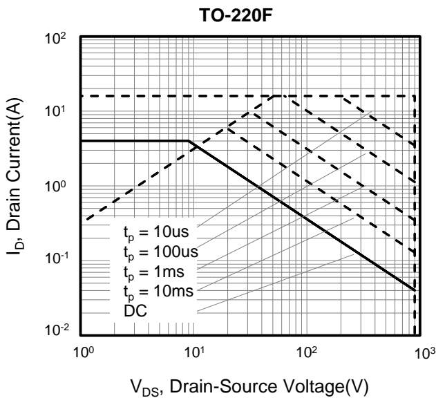
Figure 11. Safe operation area for TO-220F
