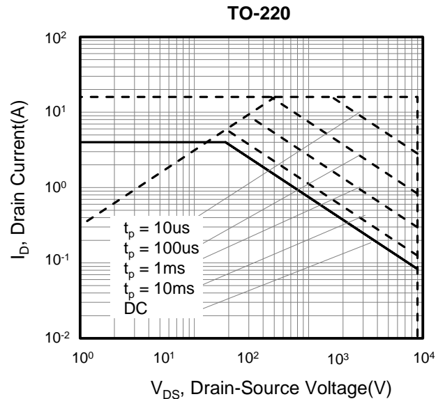
Figure 12. Safe operation area for TO-220
