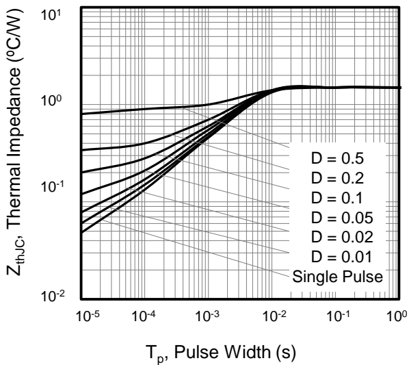
Figure 9. Transient Thermal Impedance TO-251
