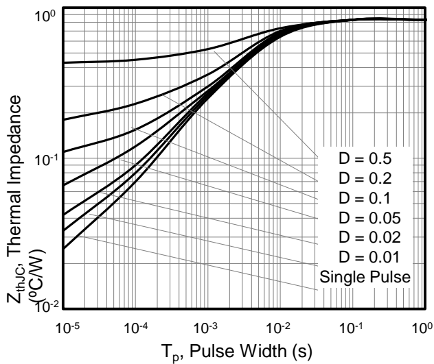
Figure 9. Transient Thermal Impedance for TO-220
