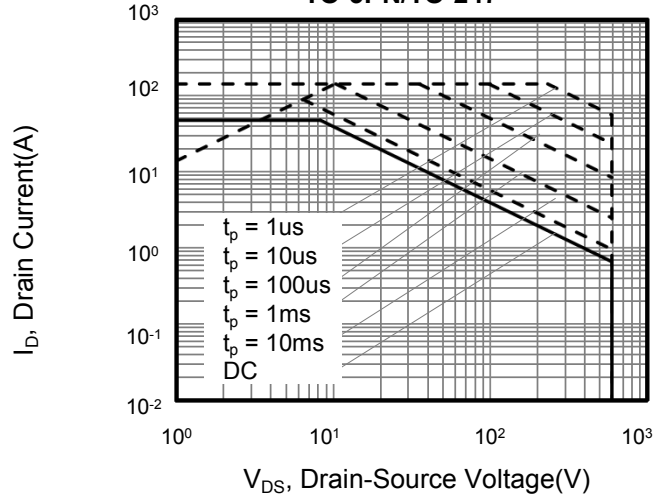
Figure 10. Safe operation area for TO-3PN/TO-247
