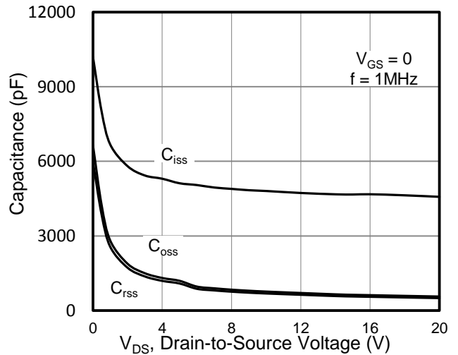
Figure 4. Capacitance
