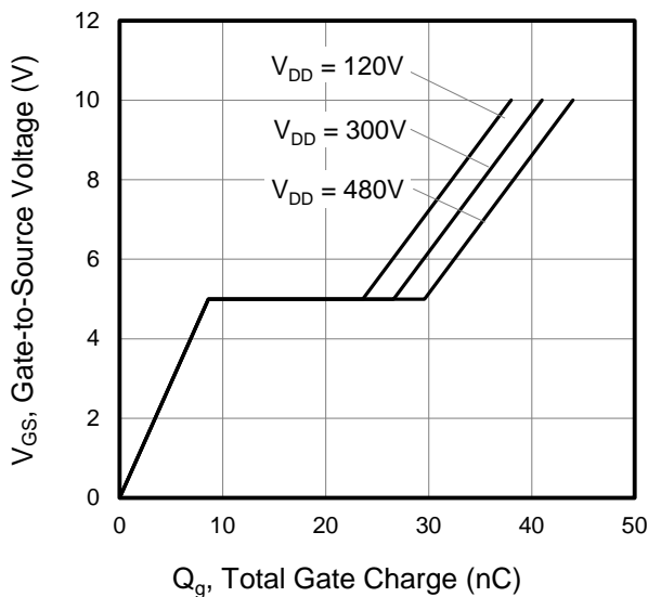
Figure 5. Gate Charge
