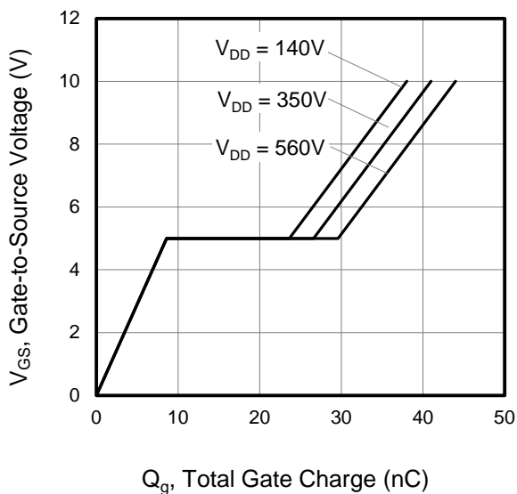
Figure 5. Gate Charge
