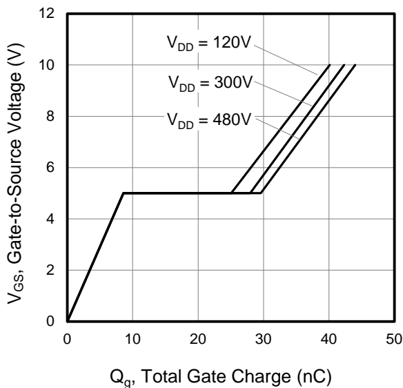
Figure 5. Gate Charge
