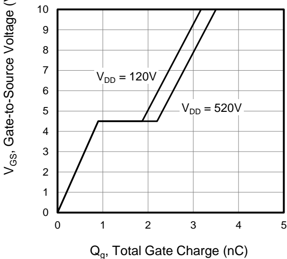
Figure 5. Gate Charge
