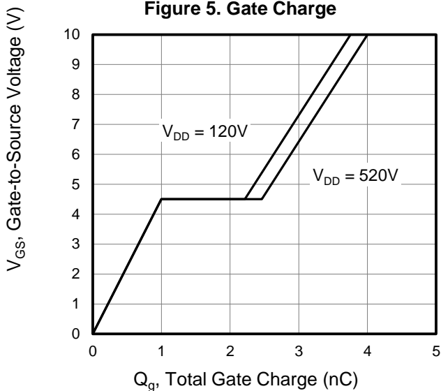
Figure 5. Gate Charge
