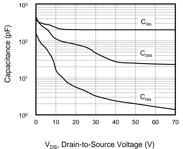
Figure 4. Capacitance
