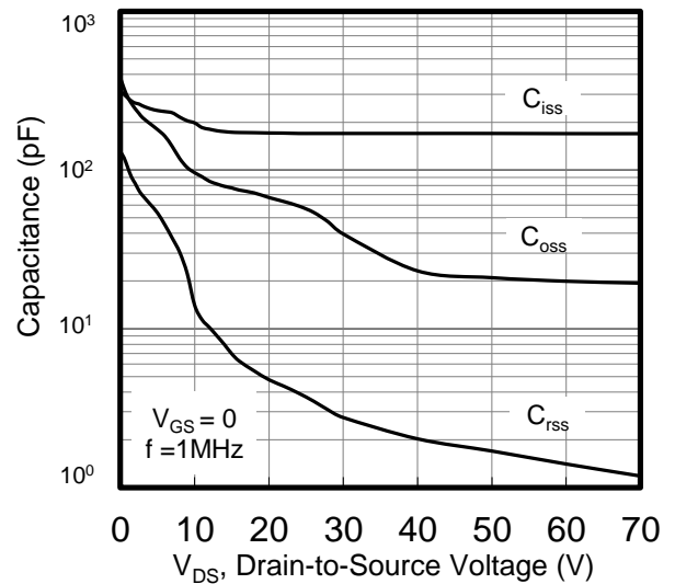
Figure 4. Capacitance
