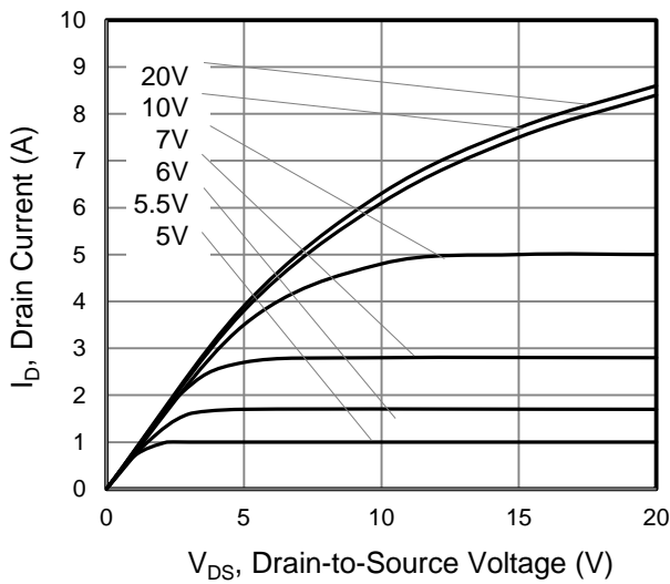
Figure 1. Output Characteristics
