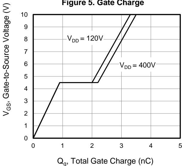
Figure 5. Gate Charge
