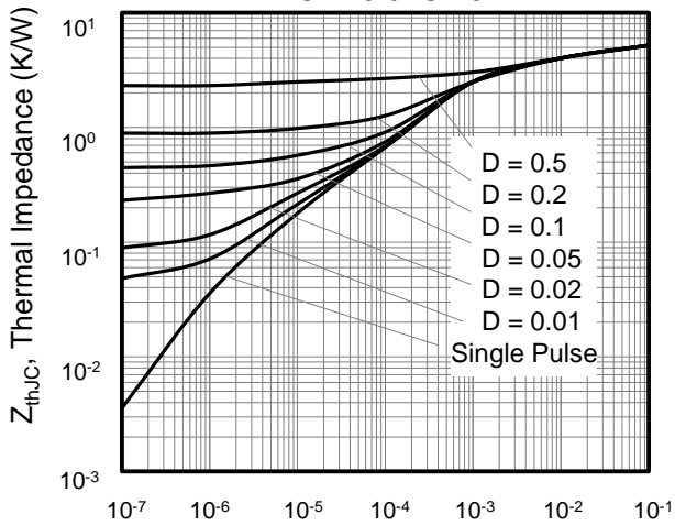
Figure 9. Transient Thermal Impedance TO-2251/TO-252
