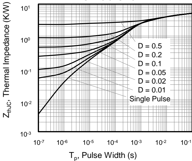
Figure 9. Transient Thermal Impedance TO-2251/TO-252
