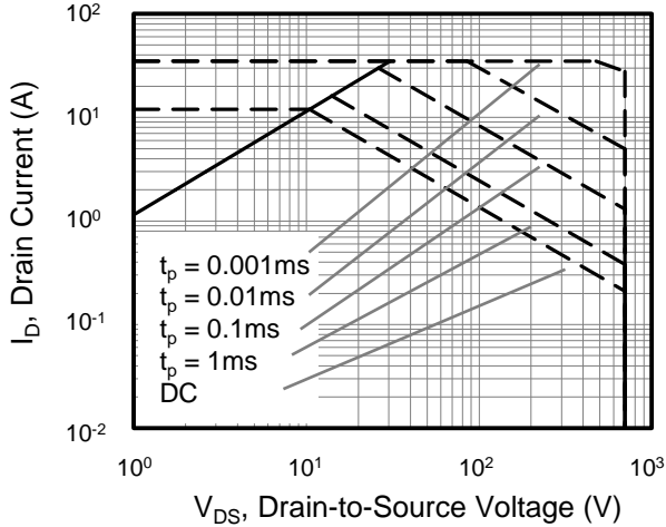
Figure 11. Safe Operating Area TO-220
